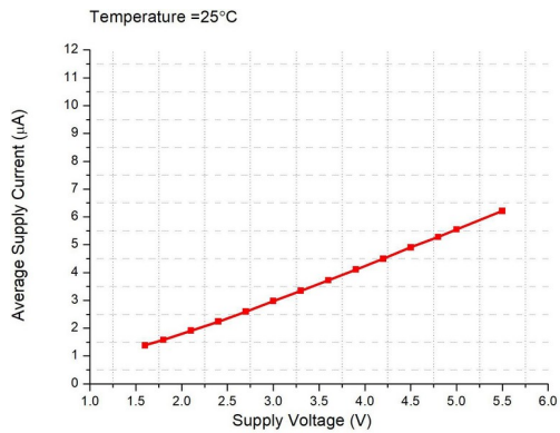
Average working current vs. supply voltage @ T A =25°C
