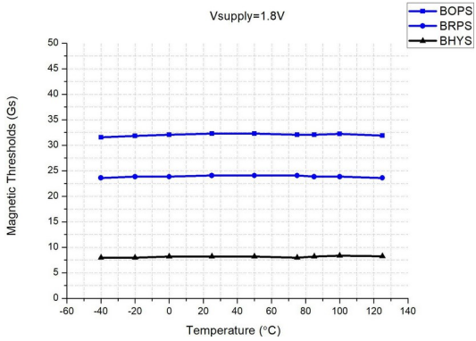
Magnetic threshold value vs temperature @ V DD =1.8V
