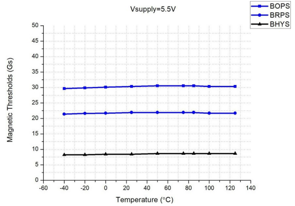
Magnetic threshold value vs temperature @ V DD =5.5V
