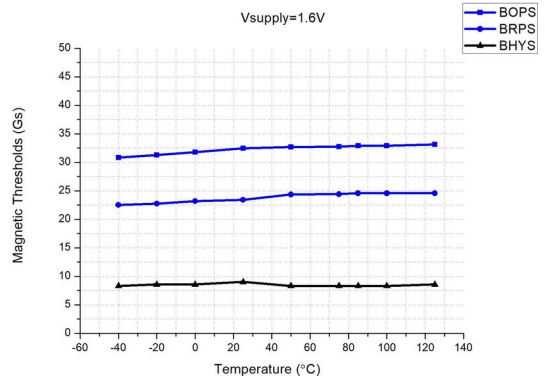
Magnetic threshold value vs temperature @ V DD =1.6V
