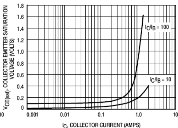
Figure 6. Collector Emitter Saturation Voltage versus Collector Current
