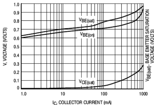
Figure 3. "On" Voltages
