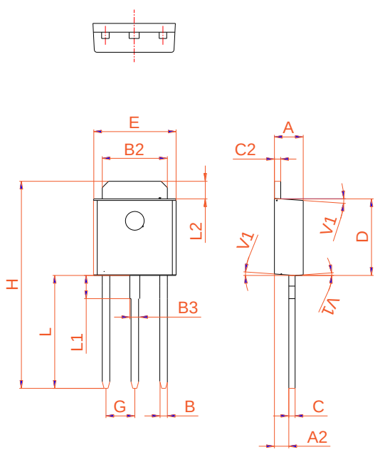
TO-251
