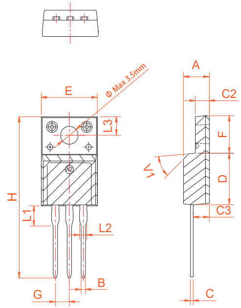
TO-220F
