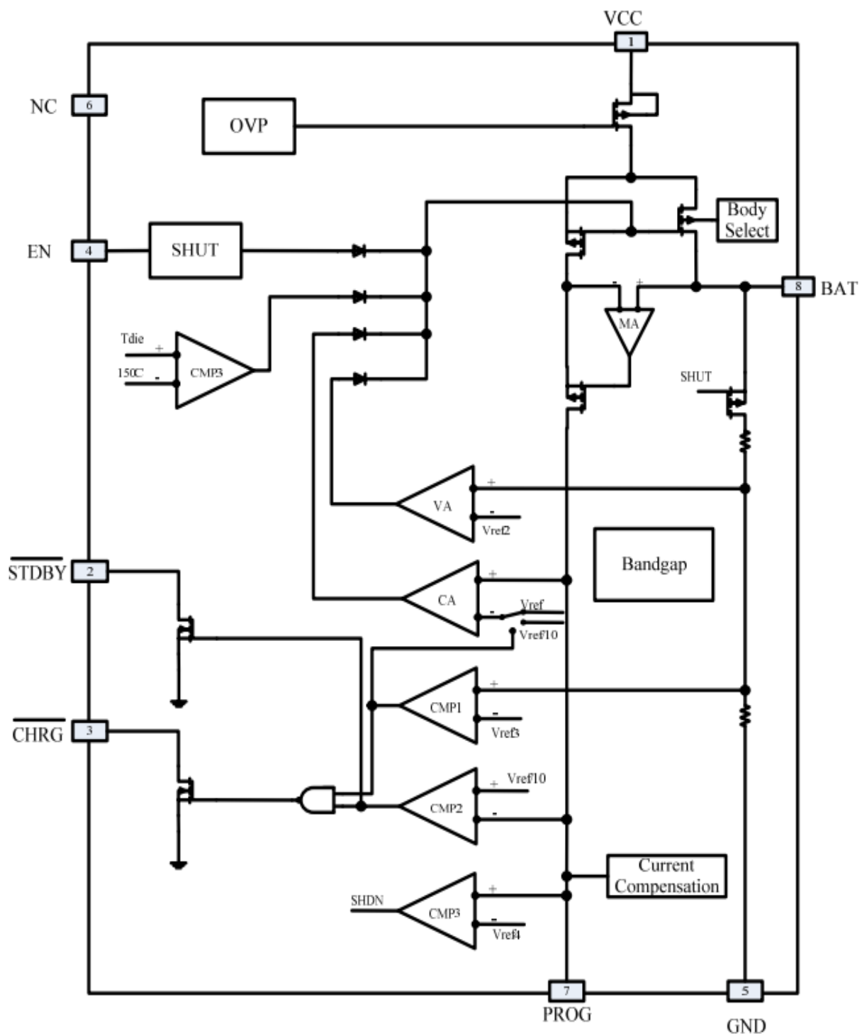
Figure3 Block Diagram
