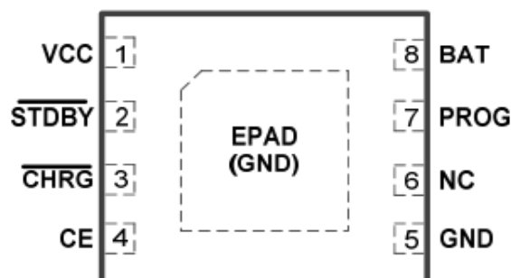
Figure 2. PIN Configuration (DFN2x2-8)
