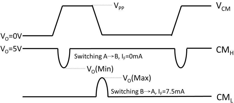
Fig.26 Waveforms of Common Mode Transient Immunity
