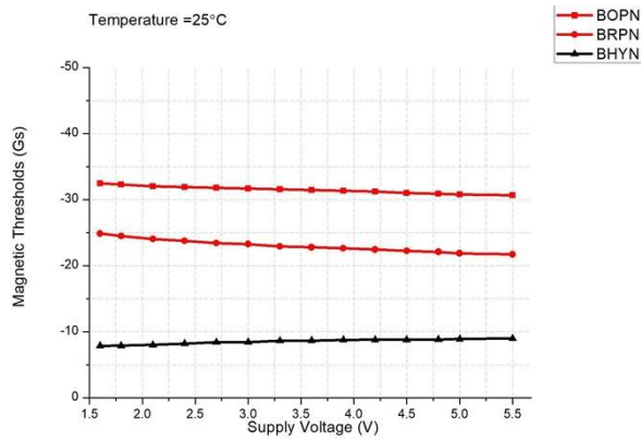
Magnetic threshold value vs. supply voltage @ T_A=25^\circ\text{C}
