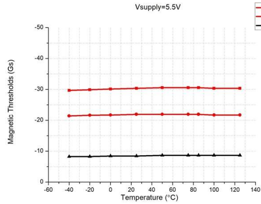
Magnetic threshold value vs temperature @ V_{DD}=5.5\text{V}
