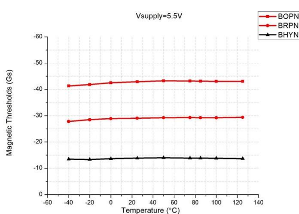
Magnetic threshold value vs temperature @VDD=5.5
