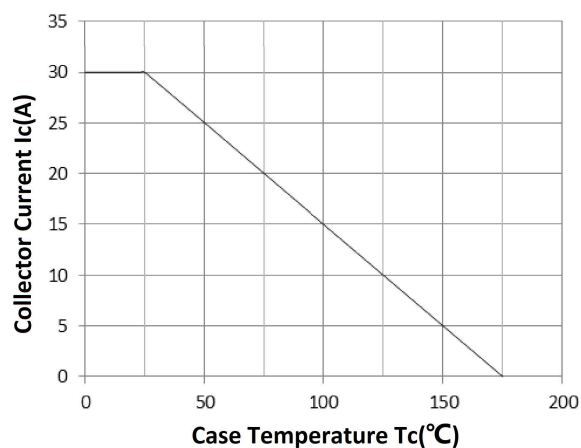
Case Temperature-Collector Current
