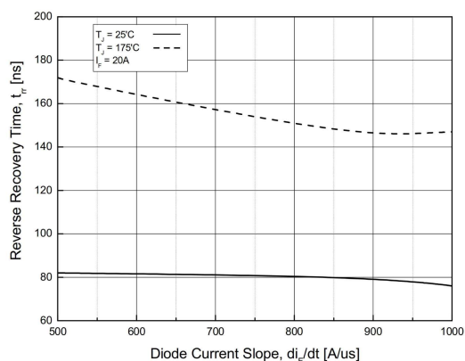
Fig.20 Reverse Recovery Time -Diode current slope
