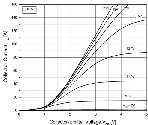
Fig.1 Typical Output Characteristics( T_J=25^\circ\text{C} )
