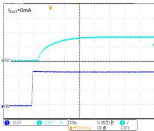
No-load start
